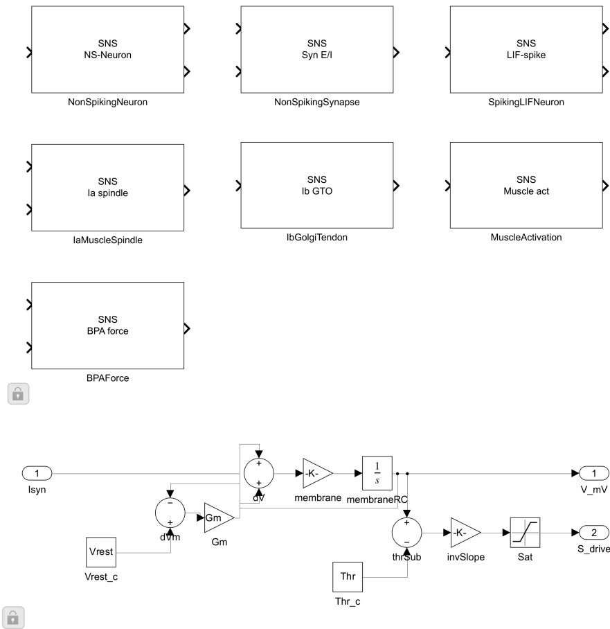
Figure 3.10: Native Simulink diagram exports showing the seven masked library blocks (top) and the internal implementation of the non-spiking neuron (bottom). The library blocks are arranged in a compact display grid for legibility. The BPA force block remains a placeholder. These implementation views do not establish quantitative knee regulation or a completed CAD-coupled Simscape Multibody plant.
