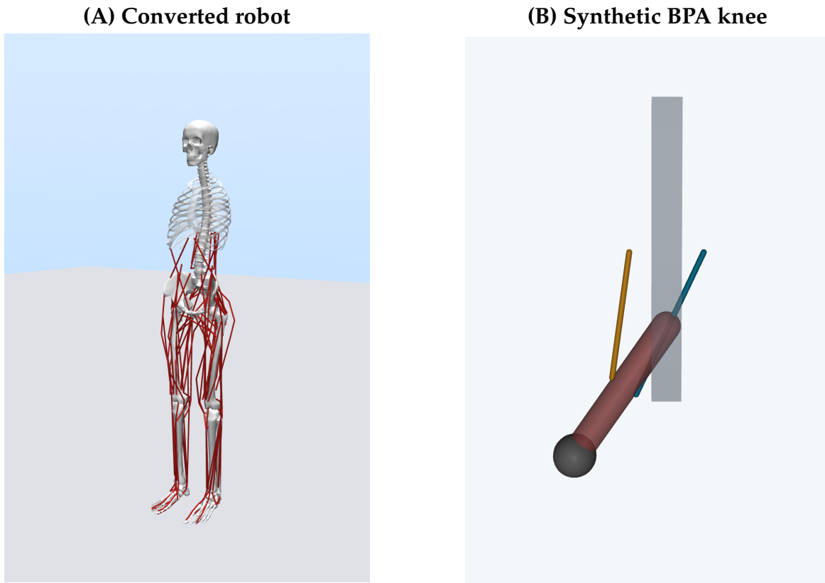
Figure 3.9: Native MuJoCo renders of (A) the converted Gait2392 robot at its saved reference pose, with muscle paths visible, and (B) the independent synthetic antagonist-BPA knee at an illustrative static angle of -35^\circ . Cyan and gold identify its named flexor and extensor tendon routes; transparency exposes the routes through the view. The models are not shown to the same scale. These views document model construction, not SNS control of the converted robot or validated torque predictions.
