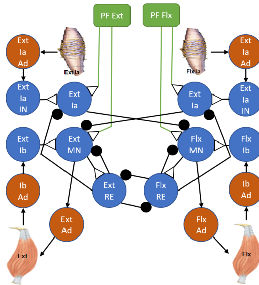
Figure 3.7: Reference schematics of (A) rhythm generation, (B) pattern formation, and (C) sensorimotor organization. Ext and Flx identify antagonist extensor and flexor pathways; IN denotes interneurons, MN motor neurons, and Ia and Ib muscle afferent pathways. Open triangles and filled circles distinguish excitatory and inhibitory synaptic connections. These schematics illustrate controller architecture and are not readouts from the phase-1 run.
